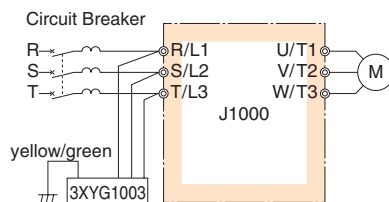
Connection Diagram
